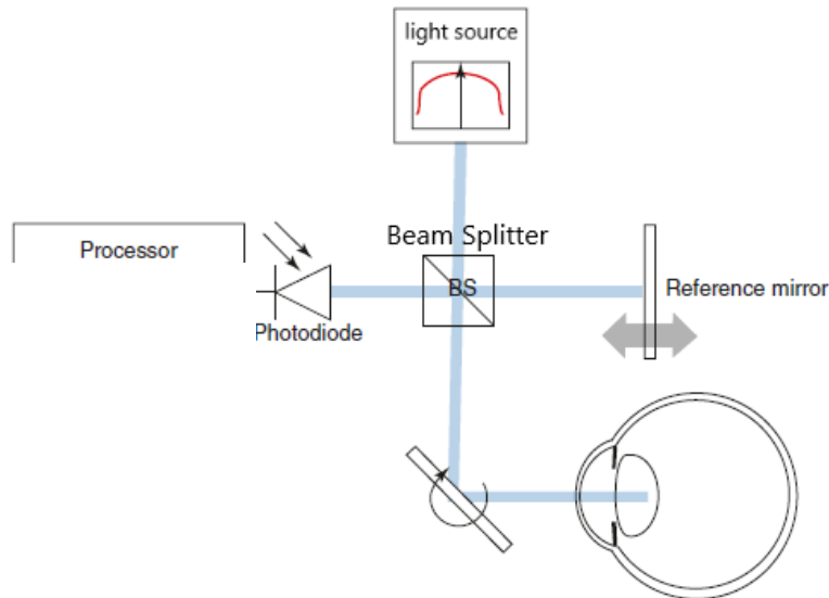
Time Domain (TD)- OCT
