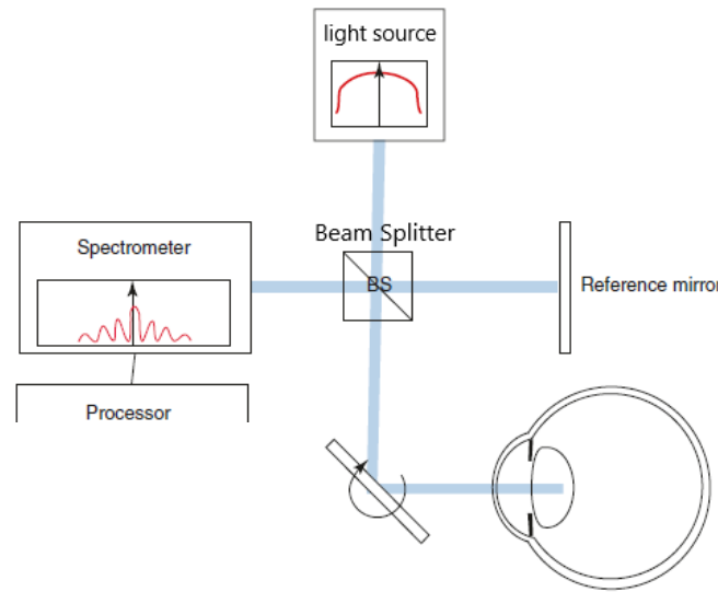
Spectral Domain (SD)- OCT
