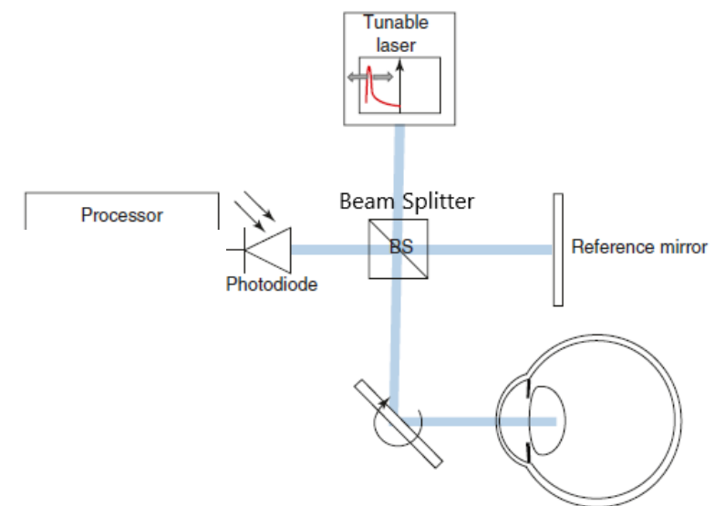
Swept Source (SS)- OCT
